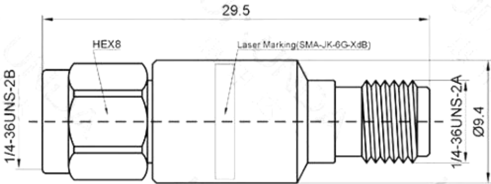
SMA Male To Female 2W 6G 10dB Fixed Attenuator
